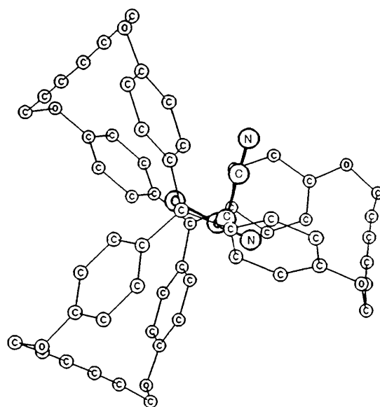
Fig. 2 View of complex 4·MeCN along its pseudo-C 3 axis. Hydrogen atoms are omitted for clarity.
