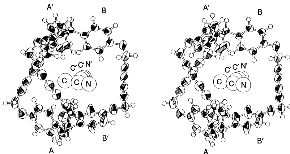
Fig. 1 ORTEP drawing of complex 4·MeCN (stereoview). The enclosed acetonitrile is found in two split positions in a 1:1 ratio.
